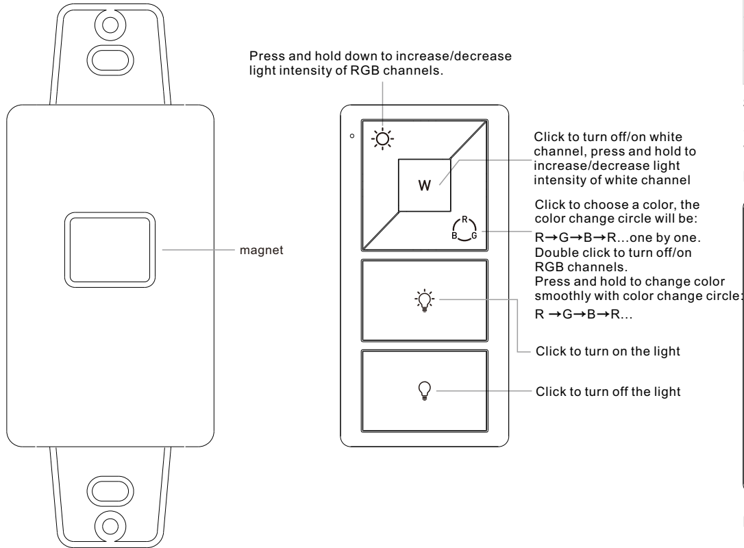
Bracket
