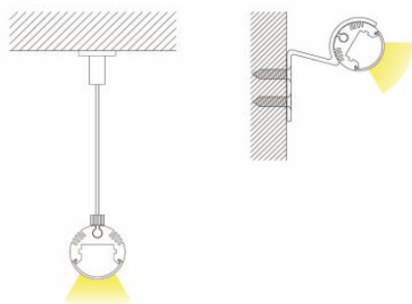
TT-20-CLIP
